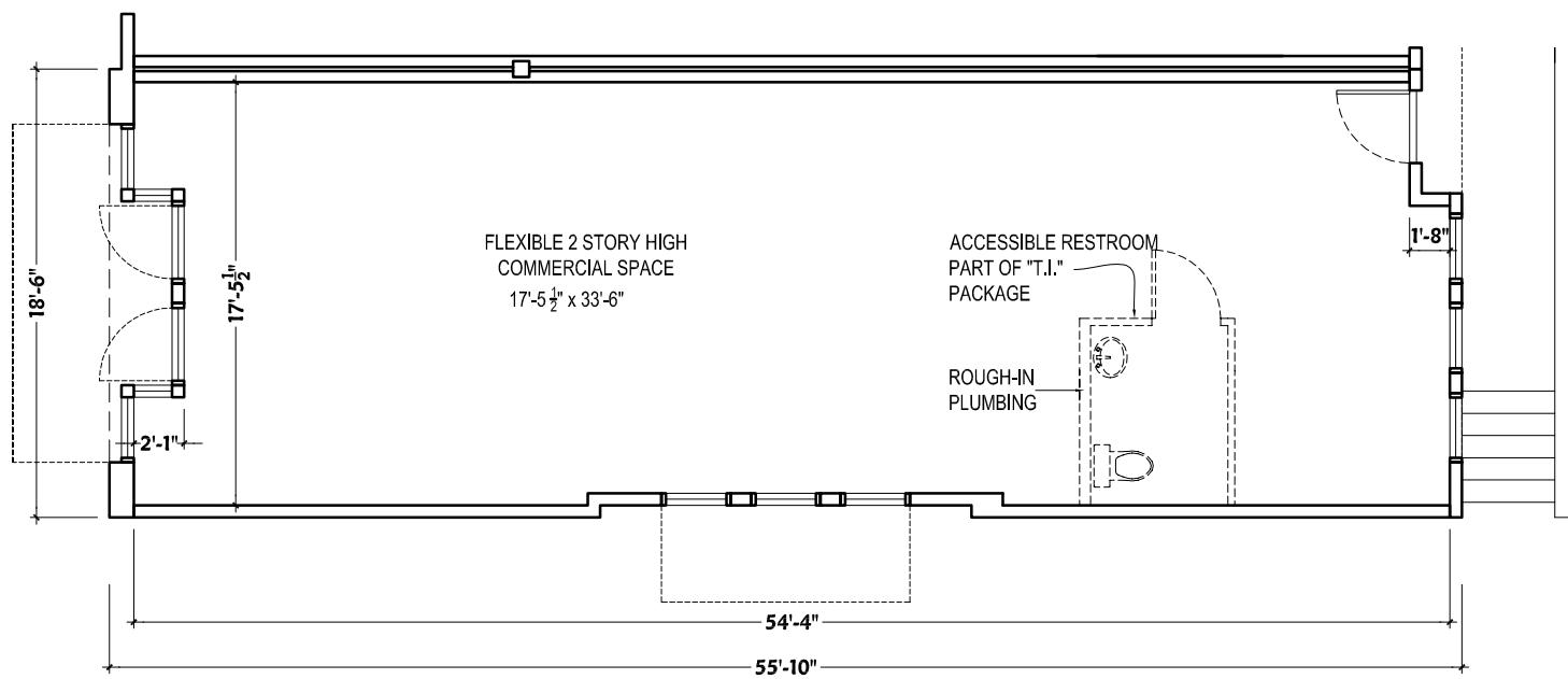
FLOOR PLAN COMMERCIAL SPACE ONLY
